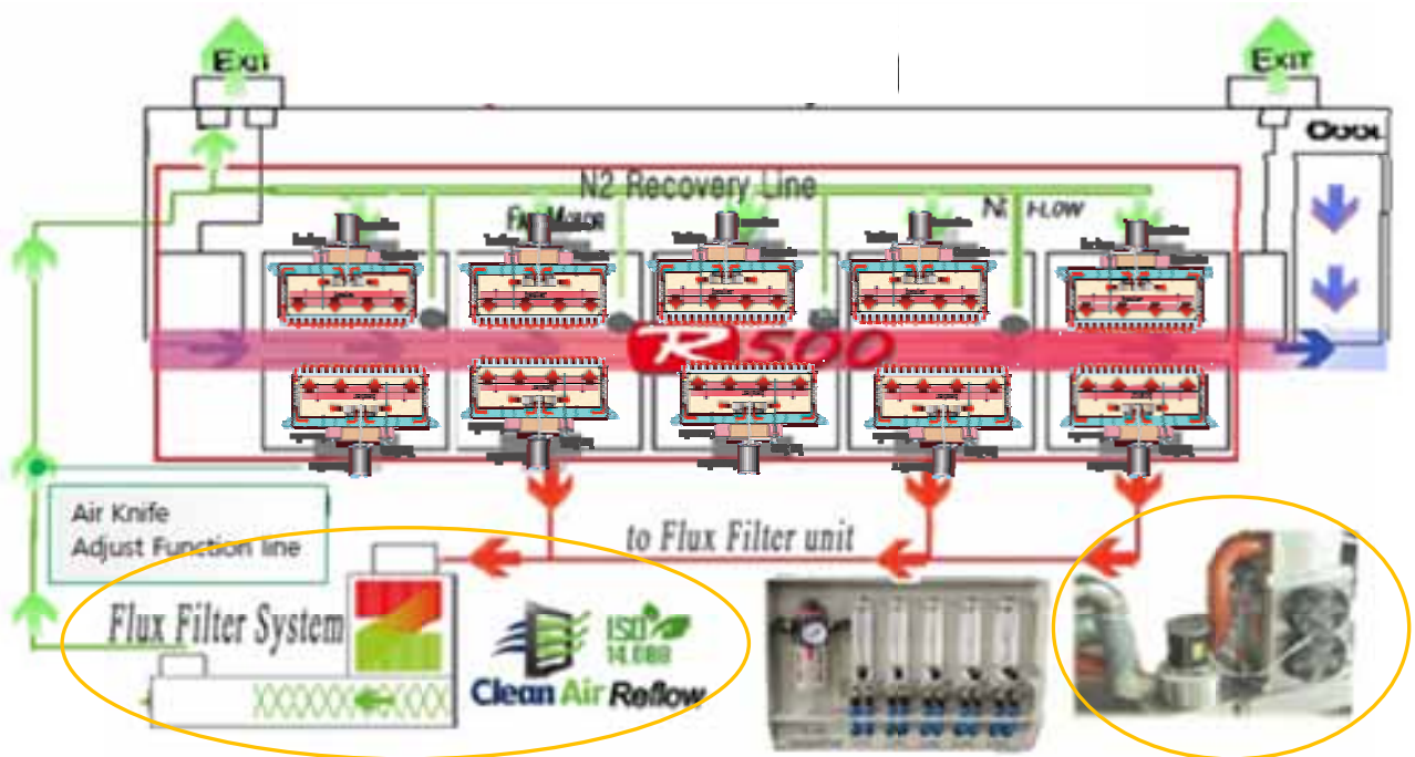
Flux Filter & N2 Recycle Flow chart
